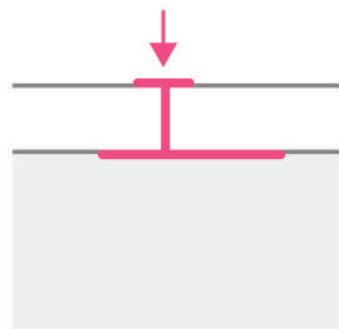
Biased I-bar
